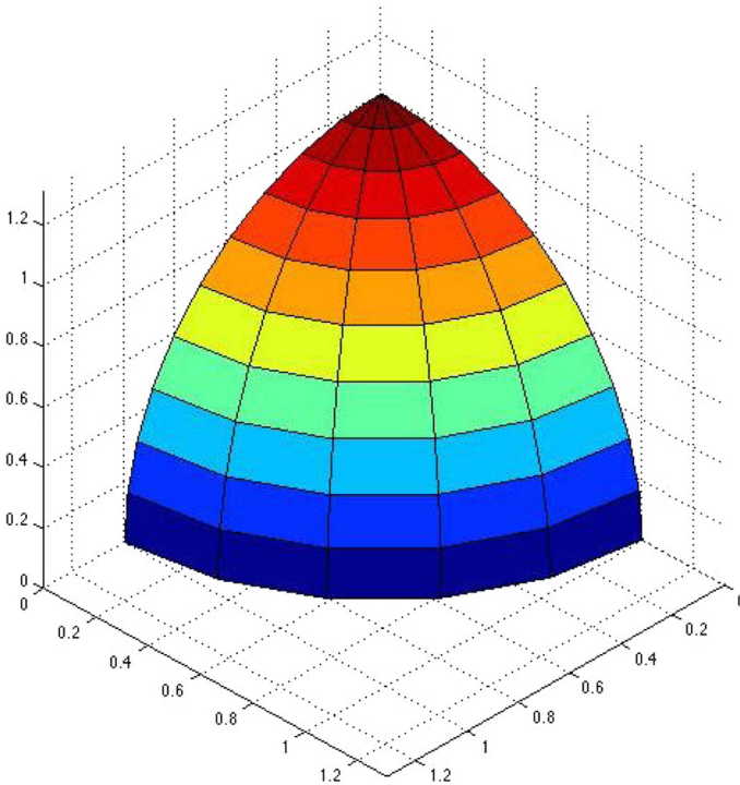
Fig. 1 The uncertainty set (1.2)
